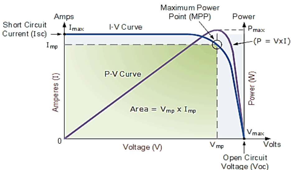
Figure 1. (I-V) Curve characteristic of solar cell.
